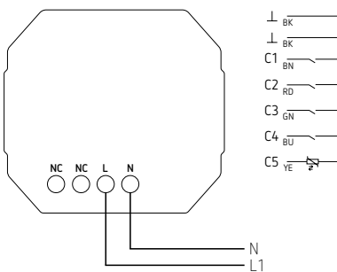
Media coupler TP-RF KNX
