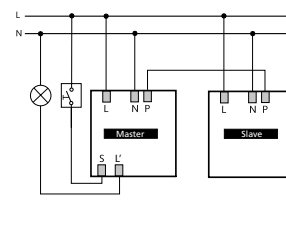
thePrema S360-100, thePrema S360 Slave
