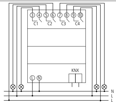
RM4 4 U KNX
